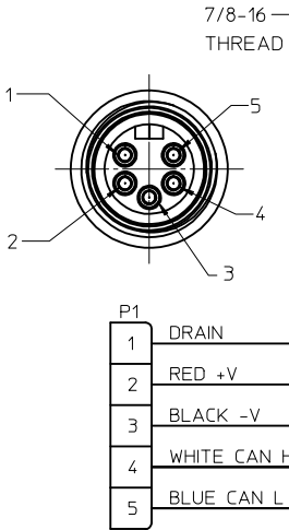
WIRING DIAGRAM
