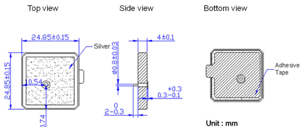
Fig. 1 Mechanical data
