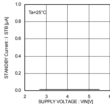
Fig.5 Standby current EN, /EN disable
