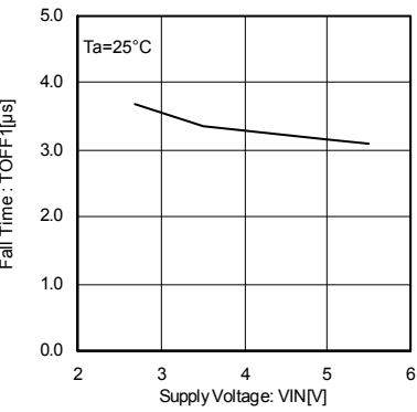
Fig.23 Output fall time
