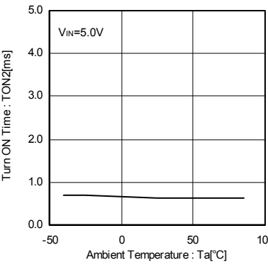
Fig.22 Output turn-on time
