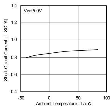
Fig.14 Short circuit current
