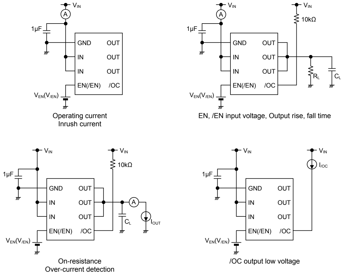
Fig.1 Measurement circuit
