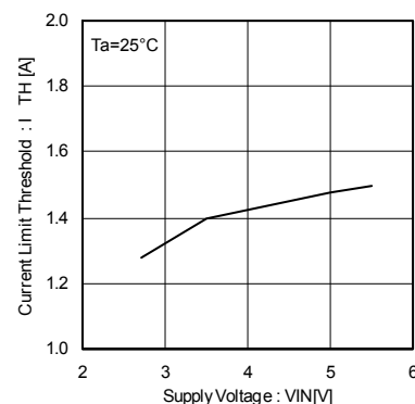
Fig.11 Current limit threshold
