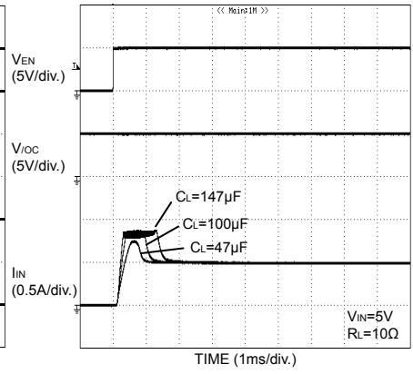
Fig.31. Inrush current response
