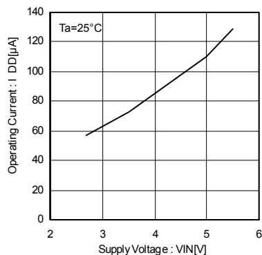
Fig.3 Operating current EN, /EN enable
