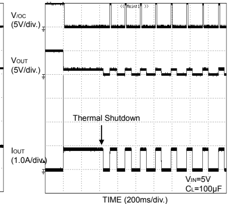
Fig.36 Thermal shutdown 1Ω load connected at enable
