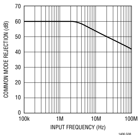
Figure 7. Common Mode Rejection vs Input Frequency
