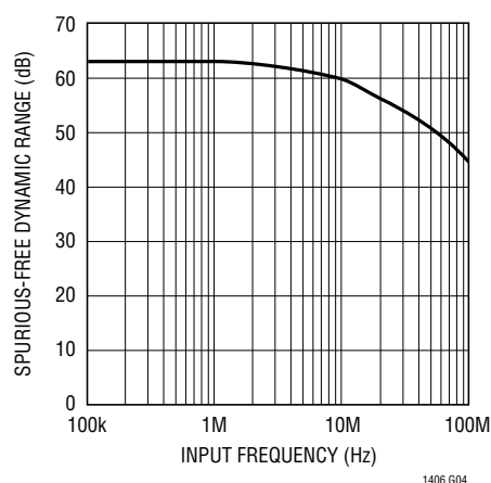
Figure 6. Spurious-Free Dynamic Range vs Input Frequency
