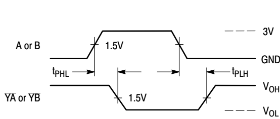
Figure 3. Switching Waveform
