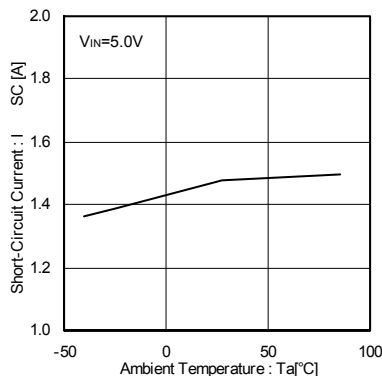
Fig.14 Short circuit current
