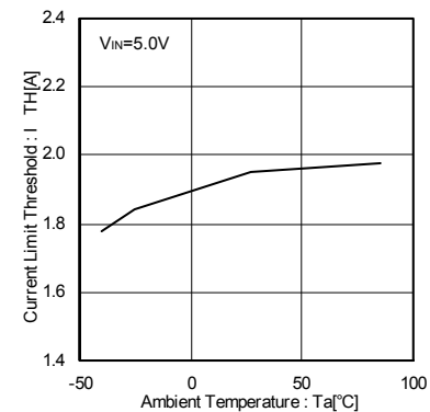
Fig.12 Current limit threshold
