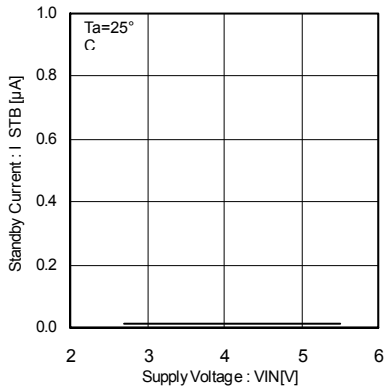
Fig.5 Standby current EN,/EN disable
