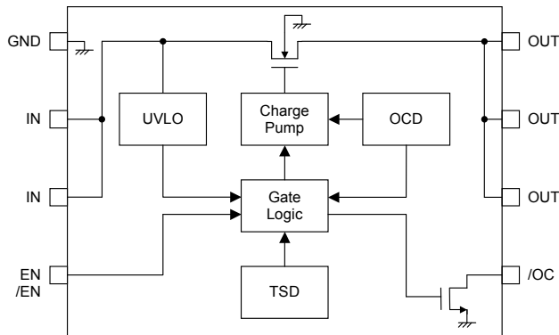
Fig.39 Block diagram
