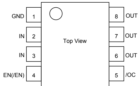
Fig.40 Pin configuration
