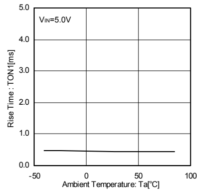
Fig.20 Output rise time
