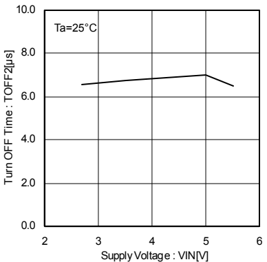
Fig.25 Output turn-off time
