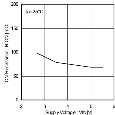
Fig.9 On-resistance
