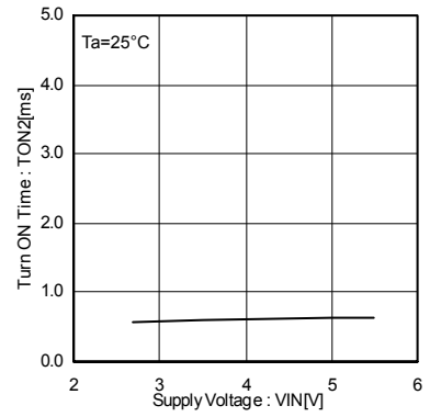
Fig.21 Output turn-on time
