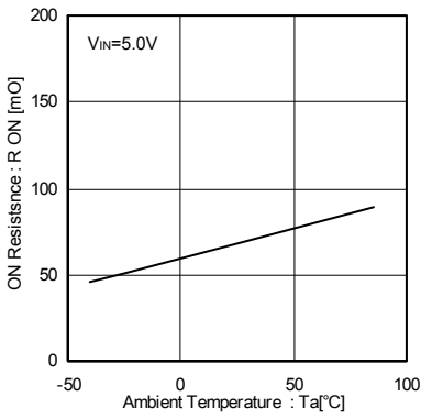
Fig.10 On-resistance
