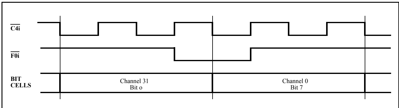
Figure 12 - Frame Alignment
