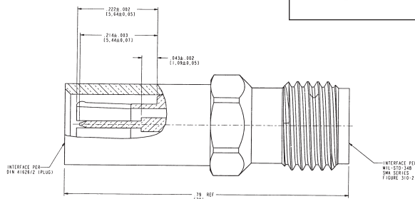
SMA Jack to 1.0/2.3 Plug 901-10006
