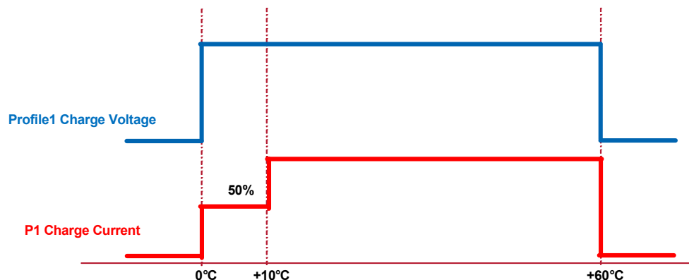
Figure 32. JEITA Profile 1
