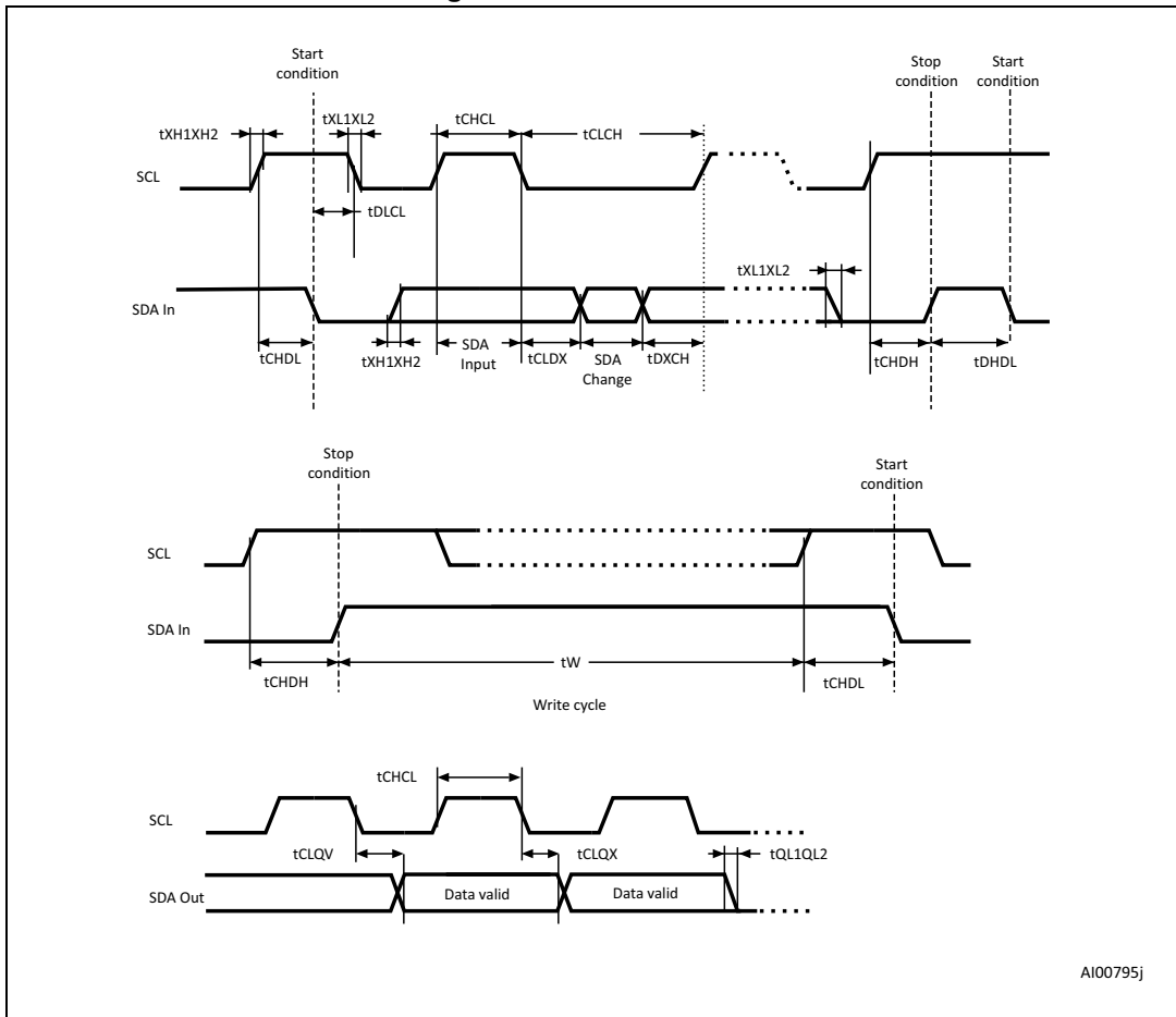
Figure 11. AC waveforms
