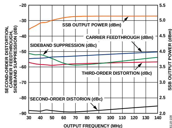
Figure 8. SSB Output Power, Second- and Third-Order Distortion, Carrier Feedthrough, and Sideband Suppression vs. Output Frequency; LO Amplitude = 0\text{ dBm}
