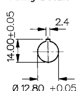
Fixing Details
