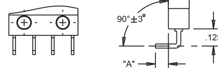
Right Angle Printed Circuit Terminal Style 5
