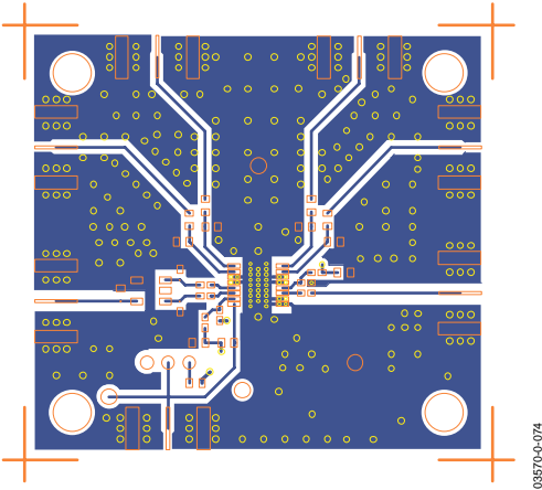
Figure 66. Layout of Evaluation Board, Top Layer
