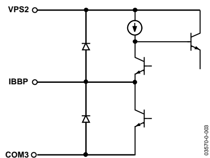
Figure 3. Circuit A
