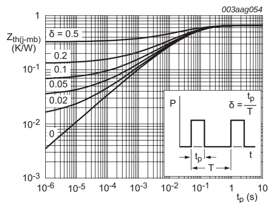
Fig 5. Transient thermal impedance from junction to mounting base as a function of pulse duration
