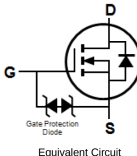
Equivalent Circuit
