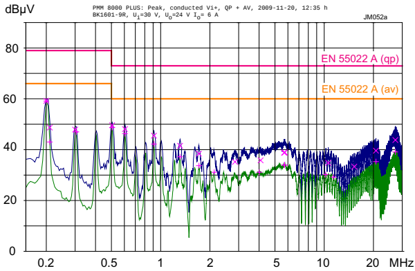
Fig. 22a Conducted emissions (peak/quasipeak and average) at the phase input according to EN 55011/22, measured at V_{i \text{ nom}} and I_{o \text{ nom}} (BK1601-9R). The neutral line performs quite similar.
