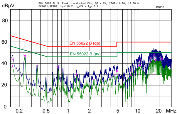
Fig. 22b Conducted emissions (peak/quasipeak and average) at the phase input according to EN 55011/22, measured at V_{i \text{ nom}} and I_{o \text{ nom}} (DK1601-9ERB1). The neutral line performs quite similar.
