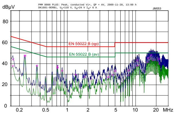
Fig. 22b Conducted emissions (peak/quasipeak and average) at the phase input according to EN 55011/22, measured at V_{i\text{ nom}} and I_{o\text{ nom}} (DK1601-9ERB1). The neutral line performs quite similar.
