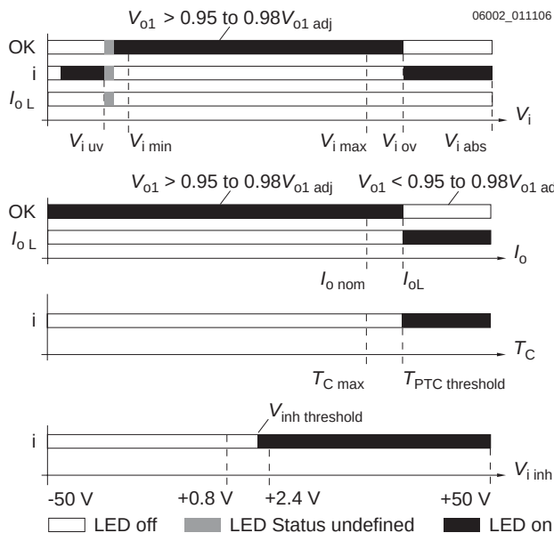
Fig. 19 LED indicators
