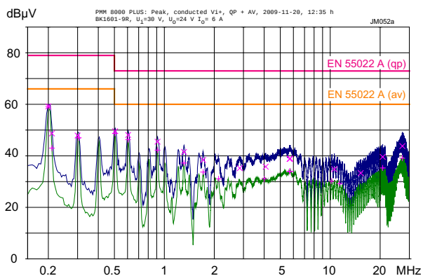
Fig. 22a Conducted emissions (peak/quasipeak and average) at the phase input according to EN 55011/22, measured at V_{i\text{ nom}} and I_{o\text{ nom}} (BK1601-9R). The neutral line performs quite similar.
