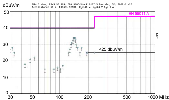
Fig. 23b Typical radiated emissions according to EN 55011/22, antenna 10 m distance, measured at V_{i\text{ nom}} and I_{o\text{ nom}} (DK1601-9ERB1)
