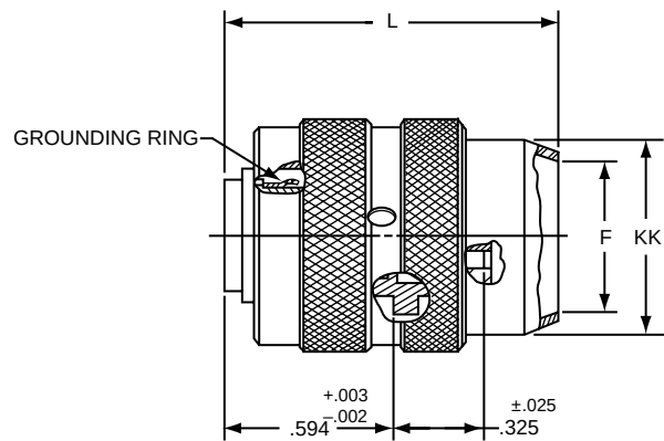
LJT06RP-XX-XXX (MS27467P)
