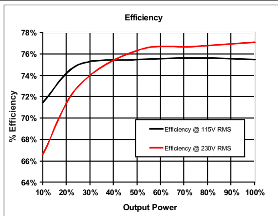
Figure 21. Efficiency
