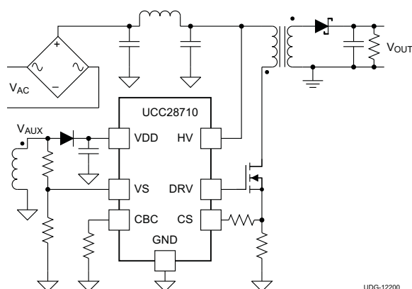
Simplified Application
