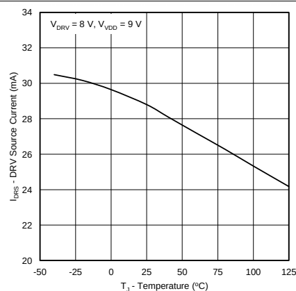
Figure 8. DRV Source Current vs. Temperature
