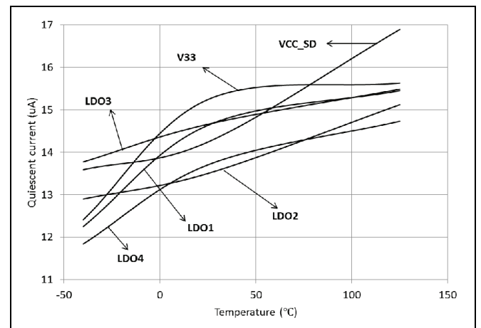
Figure 18. Quiescent current - LDOs
