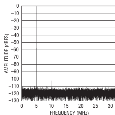
LTC2205-14: 32K Point FFT, f IN = 5.1MHz, -1dBFS, PGA = 0, DITH = 0
