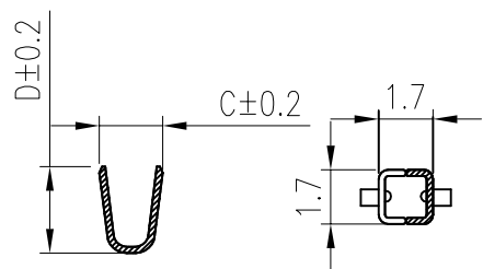
SEC C-C
