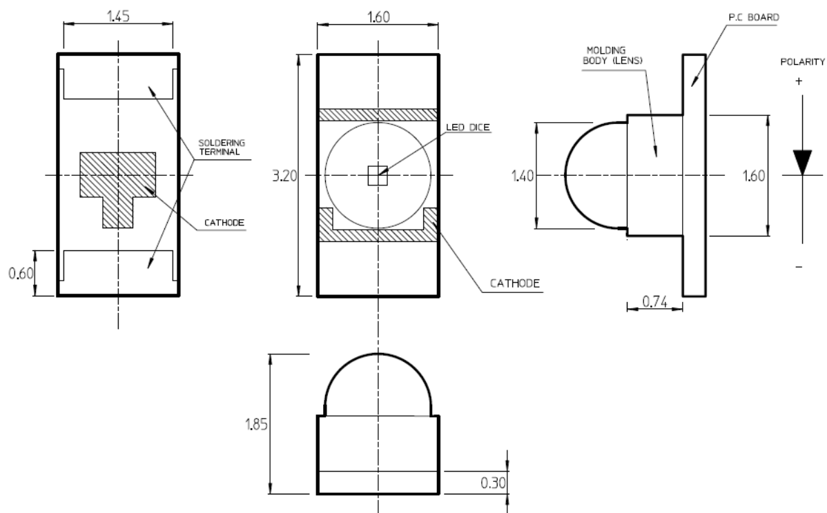
Figure 1: Package Dimensions
