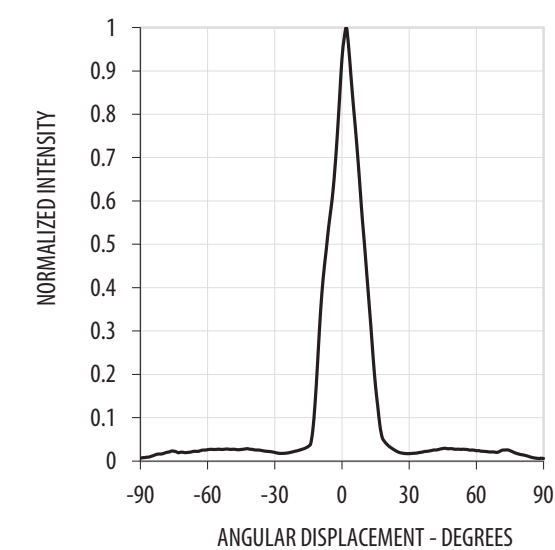
Figure 5: Radiation Pattern
