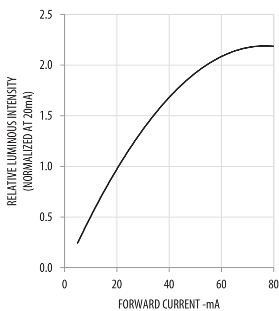
Figure 3: Luminous Intensity vs. Forward Current
