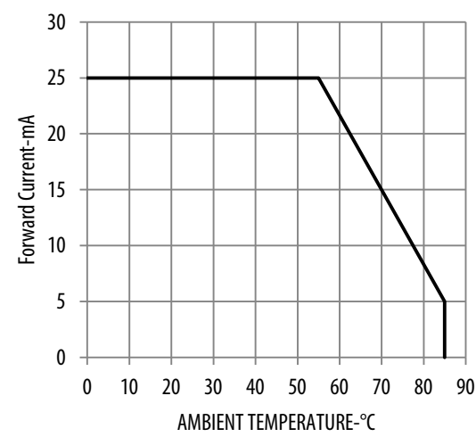
Figure 10: Derating Curve
