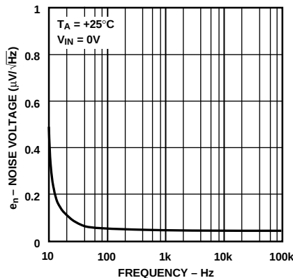
Figure 12. Voltage Noise Density vs. Frequency
