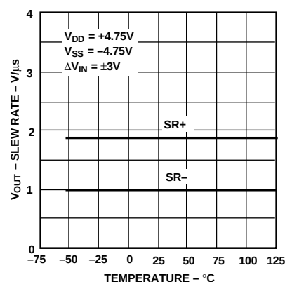
Figure 9. V_{OUT} Slew Rate vs. Temperature
