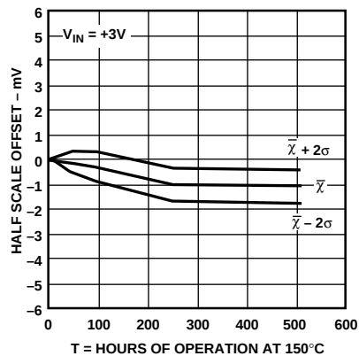
Figure 26. Output Voltage Drift Accelerated by Burn-In
