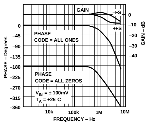
Figure 10. Gain and Phase vs. Frequency (Code = 00_H or FF_H )
