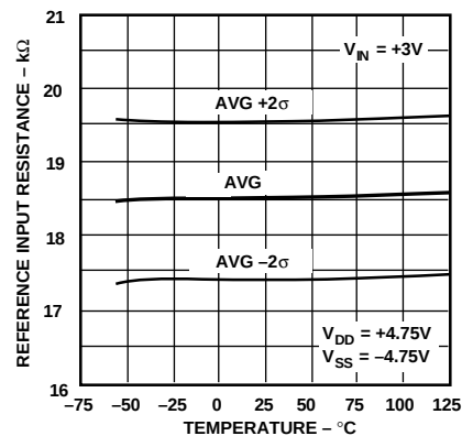
Figure 7. Input Resistance ( V_{IN} ) vs. Temperature
