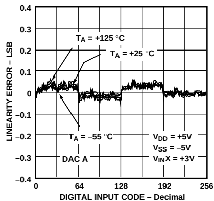
Figure 5. Linearity Error vs. Digital Code vs. Temperature
