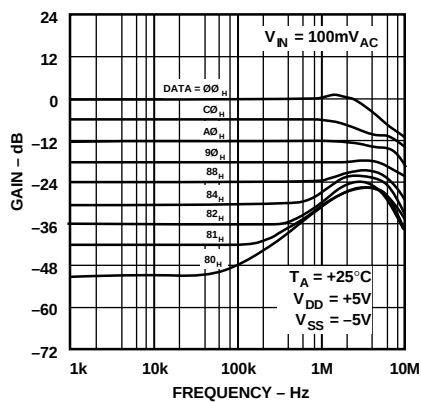
Figure 24. Gain ( V_{OUT}/V_{IN} ) and Feedthrough vs. Frequency
