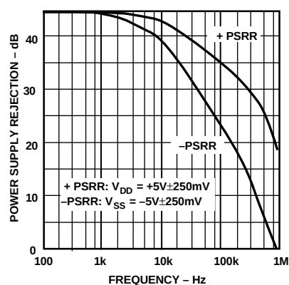
Figure 23. PSRR vs. Frequency
