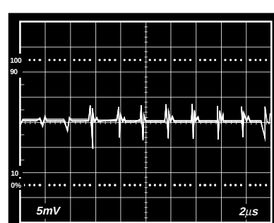
Figure 18. Clock Feedthrough— V_{OUT} @ 5 mV/Div
