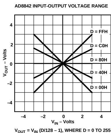
Figure 27. Functional Equivalent Circuit to the AD8842 Results in a 4-Quadrant Multiplying Channel
