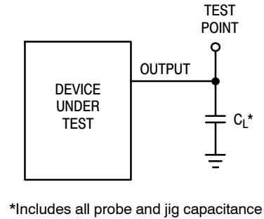
Figure 2. Test Circuit
