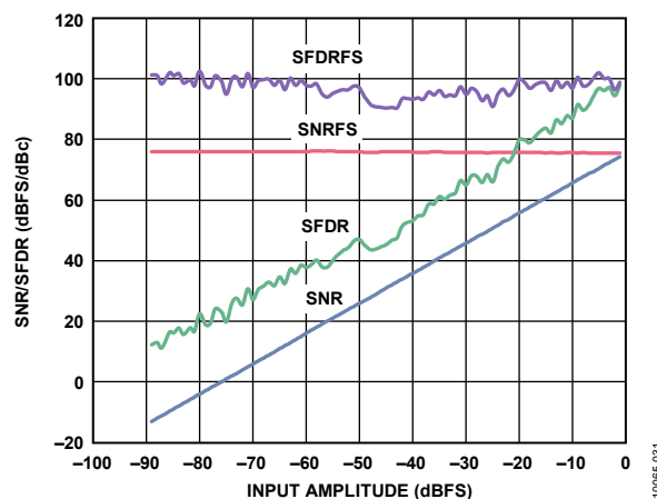
Figure 25. SNR/SFDR vs. Analog Input Level, f_{IN} = 9.7 MHz, f_{SAMPLE} = 105 MSPS
