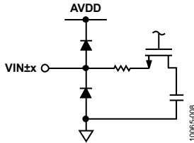
Figure 47. Equivalent Analog Input Circuit
