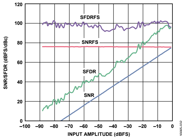
Figure 36. SNR/SFDR vs. Analog Input Level, f_{IN} = 9.7 MHz, f_{SAMPLE} = 125 MSPS
