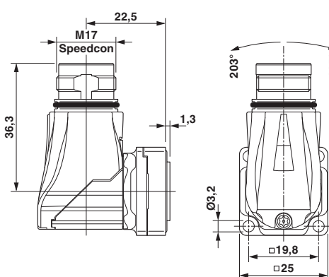
Dimensional drawing
