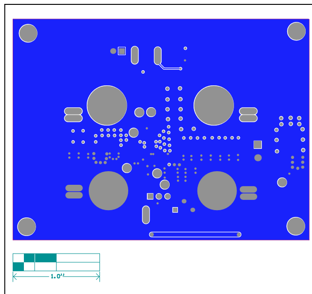
Figure 6. MAX15090B EV Kit PCB Layout—Solder Side
