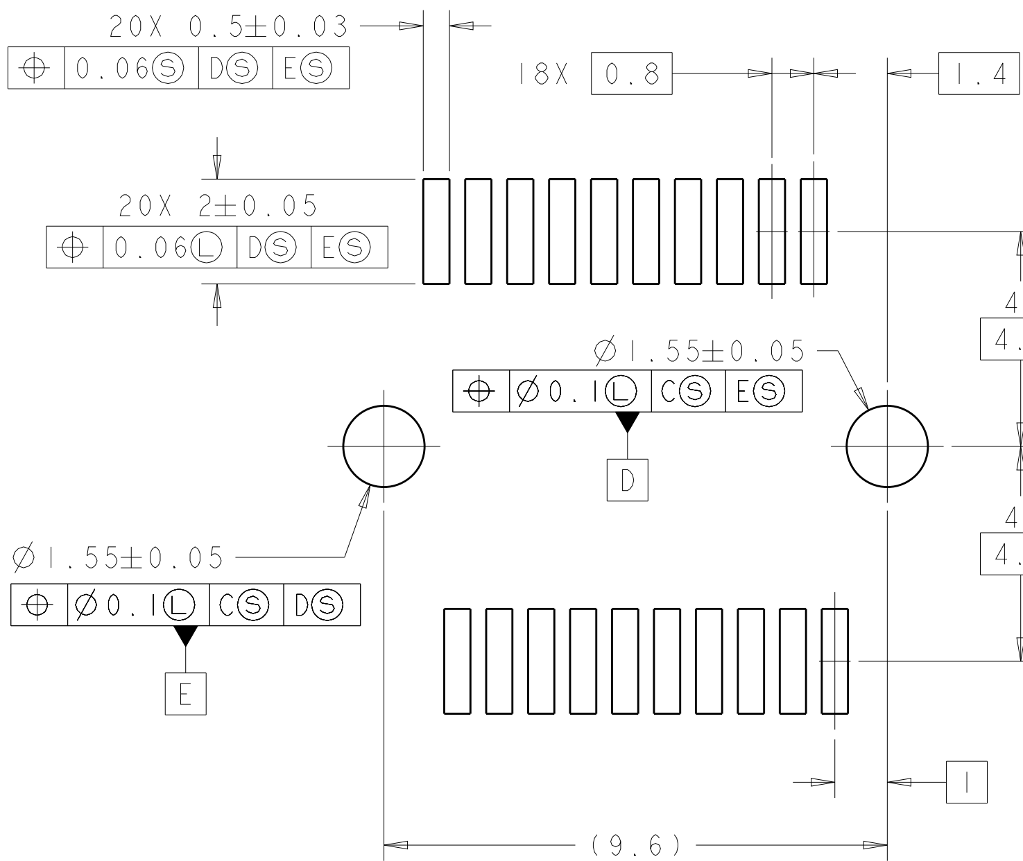
DETAIL F SCALE 10:1
