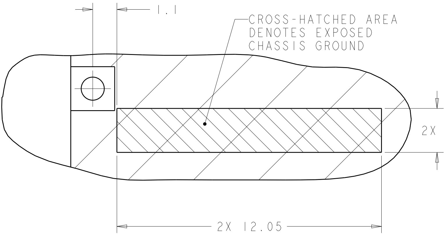
DETAIL G SCALE 10:1
