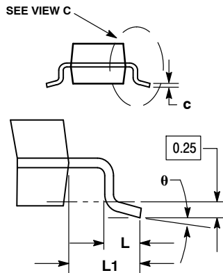
VIEW C
