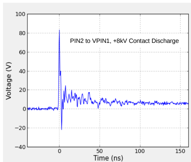
Figure 8 ESD Response to IEC 61000-4-2
