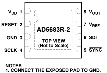
Figure 8. Pin Configuration, 8-Lead LFCSP, \overline{\text{RESET}} Option
