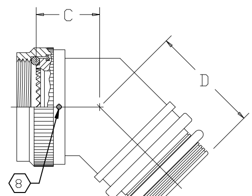
45° ADAPTER-TYPE I
