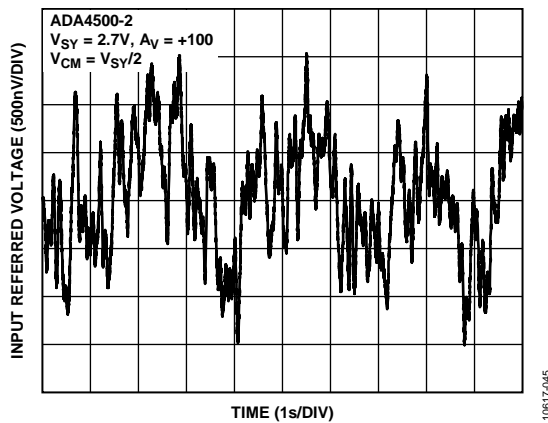
Figure 51. 0.1 to 10 Hz Noise, V_{SY} = 2.7\text{V}
