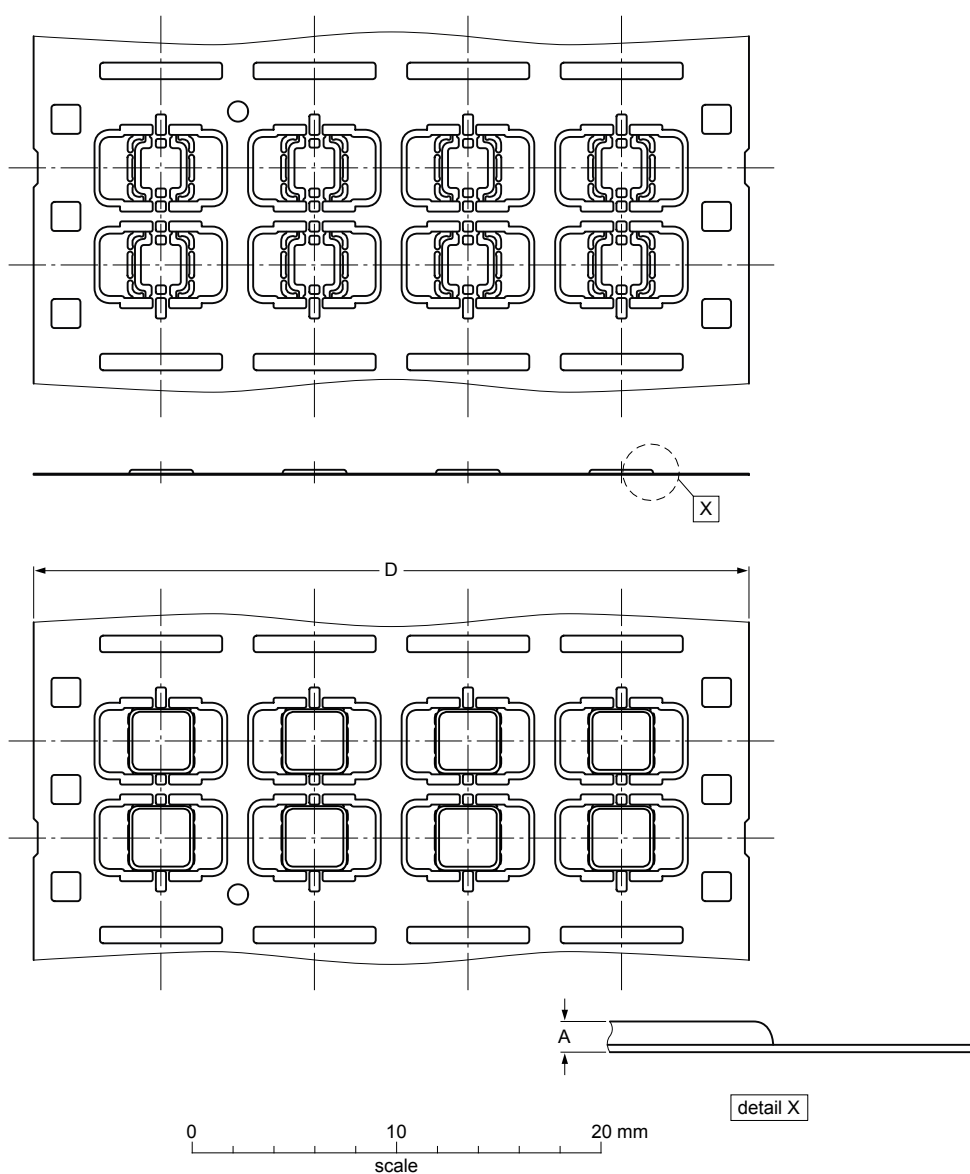
PLLMC: plastic leadless module carrier package; 35 mm wide tape
