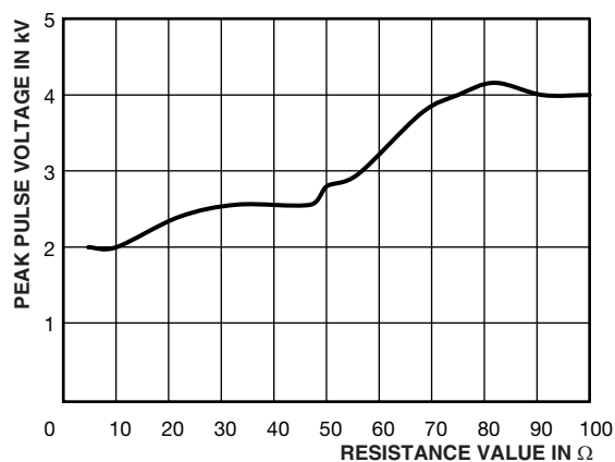
PEAK PULSE VOLTAGE LIMIT FOR AC03-CS
