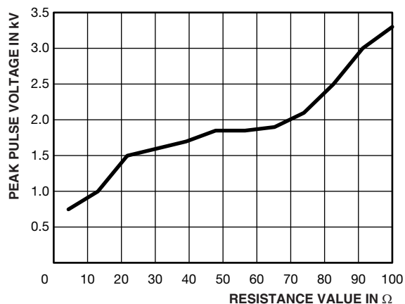
PEAK VOLTAGE LIMIT FOR AC01-CS
