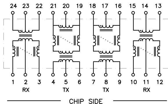
CHIP SIDE
