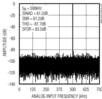
FFT PLOT (MAX1077)
