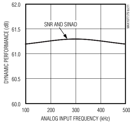
DYNAMIC PERFORMANCE vs. INPUT FREQUENCY (MAX1079)
