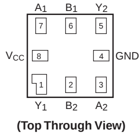
Pad Assignments for MicroPak
