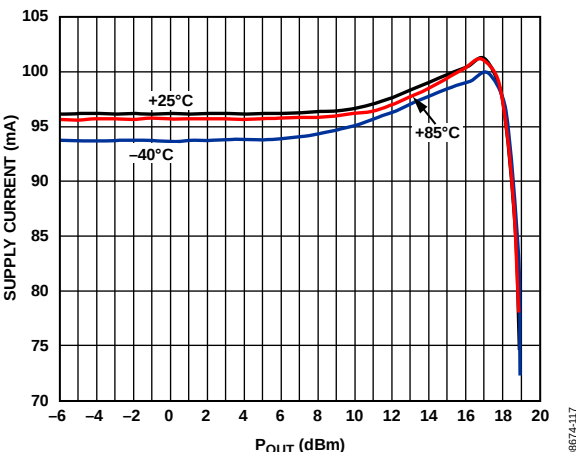
Figure 15. Supply Current vs. P_{OUT} at Various Temperatures
