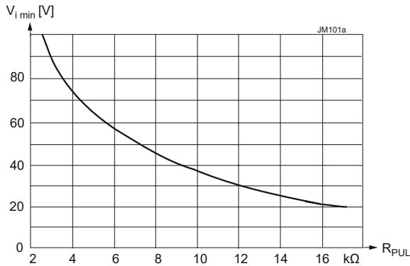
Fig. 3 R_{PUL} versus switch-on voltage (HR models)
