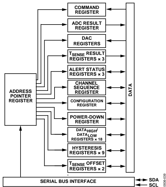
Figure 46. Register Structure
