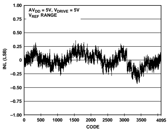
Figure 13. ADC INL, Differential Input, V_{REF} Range
