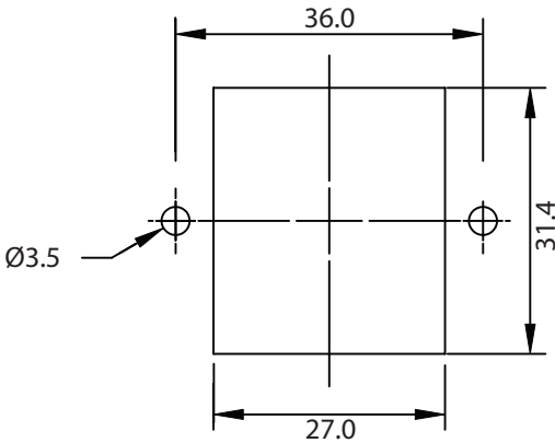
PANEL CUTOUT
