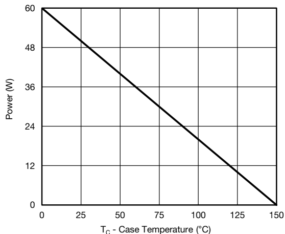
Power, Junction-to-Case
