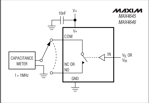
Figure 5. Channel Off/On-Capacitance
