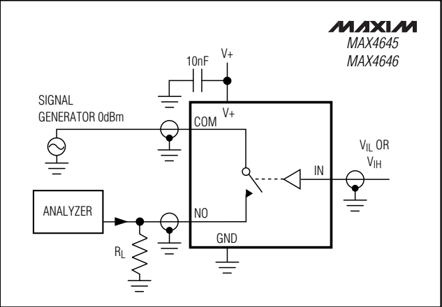
Figure 4. Off-Isolation/On-Channel Bandwidth
