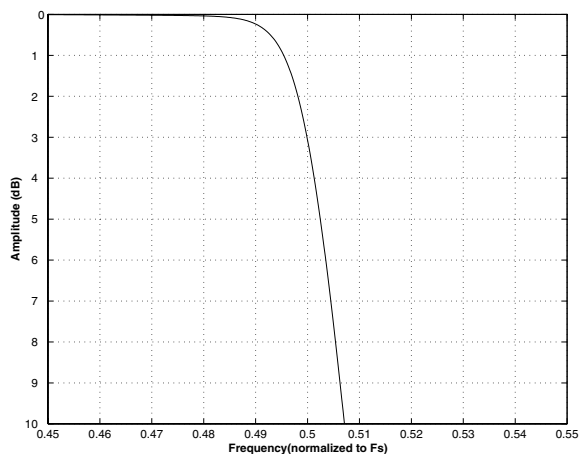
Figure 14. Single Speed (fast) Transition Band (detail)
