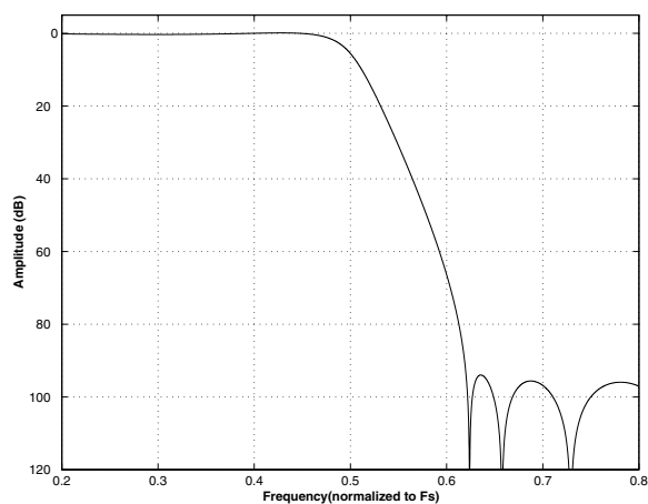
Figure 29. Quad Speed (fast) Transition Band
