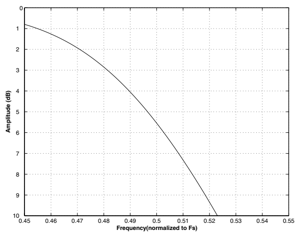
Figure 34. Quad Speed (slow) Transition Band (detail)
