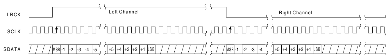
Figure 4. Format 0, Left Justified up to 24-Bit Data
