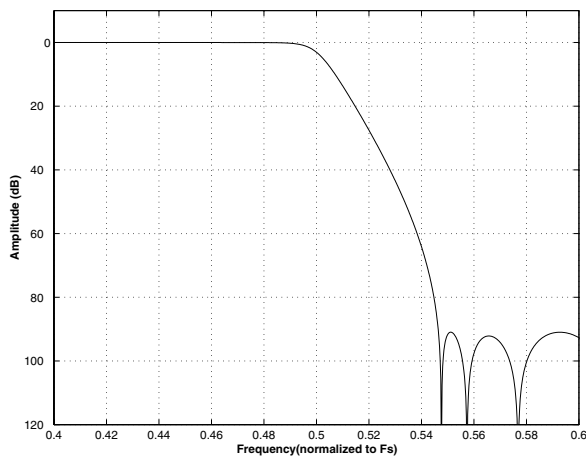
Figure 13. Single Speed (fast) Transition Band
