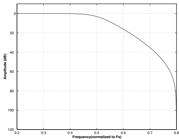
Figure 25. Double Speed (slow) Transition Band
