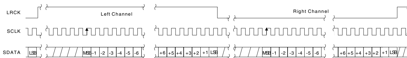
Figure 6. Format 2, Right Justified 16-Bit Data
