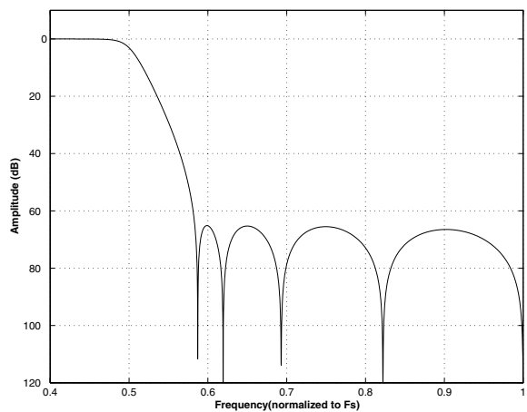
Figure 16. Single Speed (slow) Stopband Rejection
