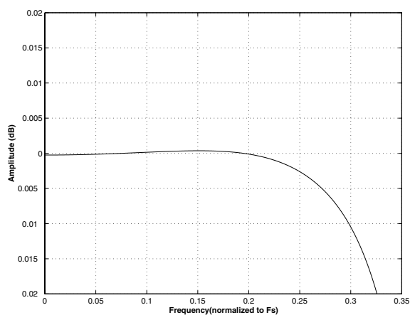
Figure 27. Double Speed (slow) Passband Ripple
