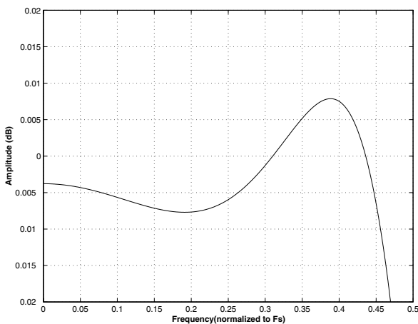
Figure 15. Single Speed (fast) Passband Ripple
