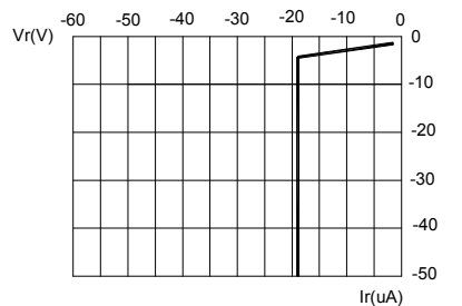
FIG.3a BLUE & GREEN REVERSE CURRENT VS. REVERSE VOLTAGE.
