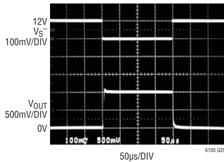
Step Response V_{SENSE} = 0V to 100mV , V_S^+ = 12V
