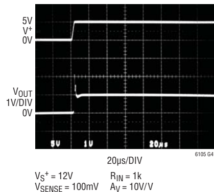
Power Supply Start-Up Response
